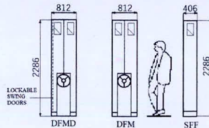
SYSTEM A & SYSTEM B FRONT ELEVATION
