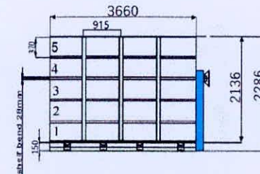
SYSTEM B 4 BAYS MOBILE COMPACTOR
